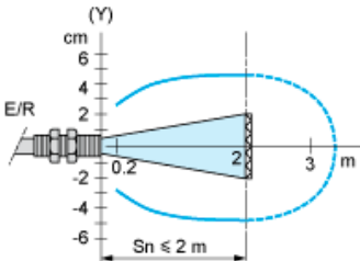
(Y) Ø of beam With reflector XUZY50
